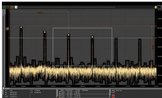
Use the FFT mask to test frequency margins and capture rare events.
